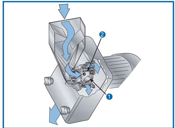
COMITROL® PROCESSOR MODEL 3600 SLANT
