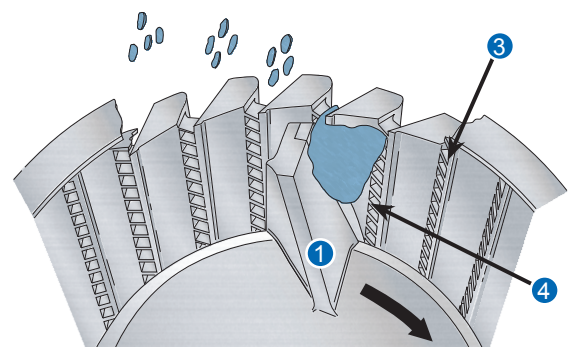
CUTTING HEAD ASSEMBLY
